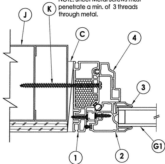
4 HORIZONTAL CROSS SECTION 2 Metal Stud Construction
