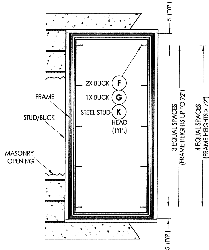
FRAME ANCHORING
